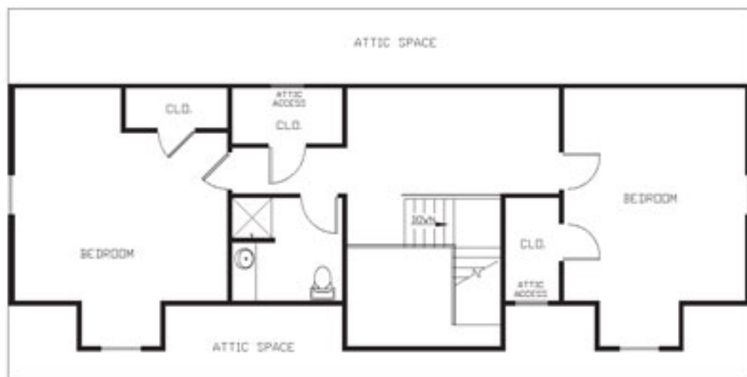
Suggested Second Floor Layout
