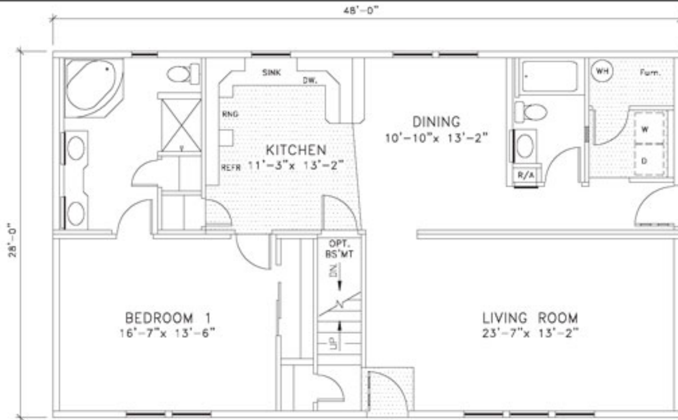
Suggested Second Floor Layout
